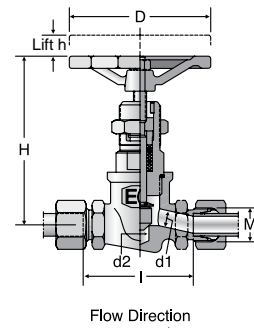
Flow Direction External threaded spindle and body of low grade forged stainless steel
